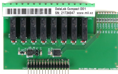
Modul DataLab Compact D01
