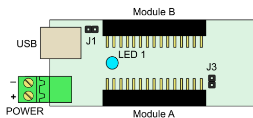
CPU modul DL-CPU2
