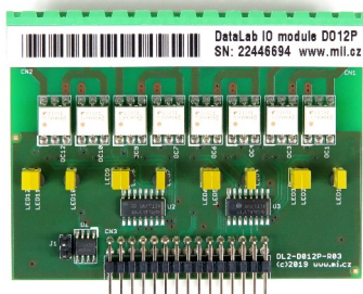
Modul DataLab DO12
